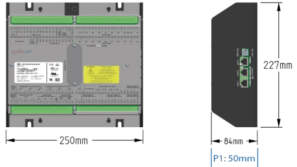
Metal housing for cabinet mounting
