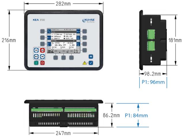
Plastic housing for front panel mounting
