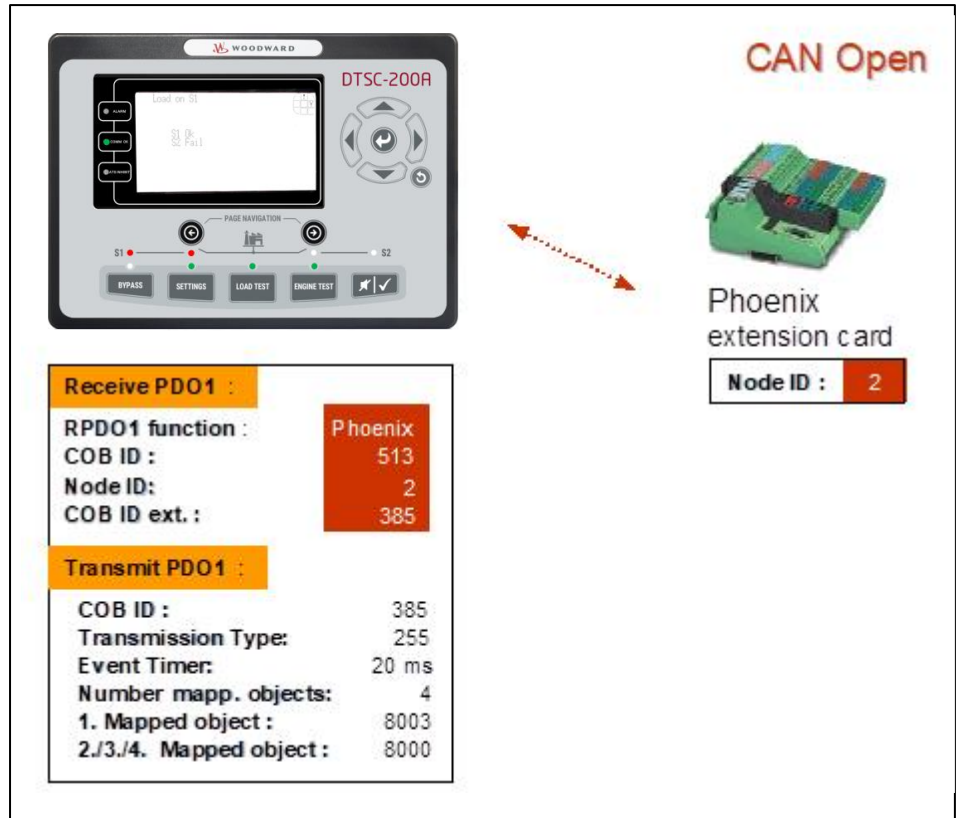
Figure 4-6: CANopen interface - expansion with Phoenix terminal
