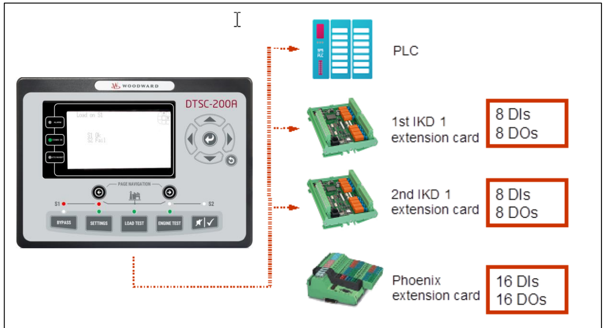
Figure 4-3: CANopen interface - external devices
