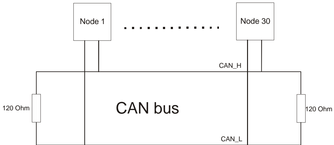
Figure 1-4: Interface - The CAN bus loop
