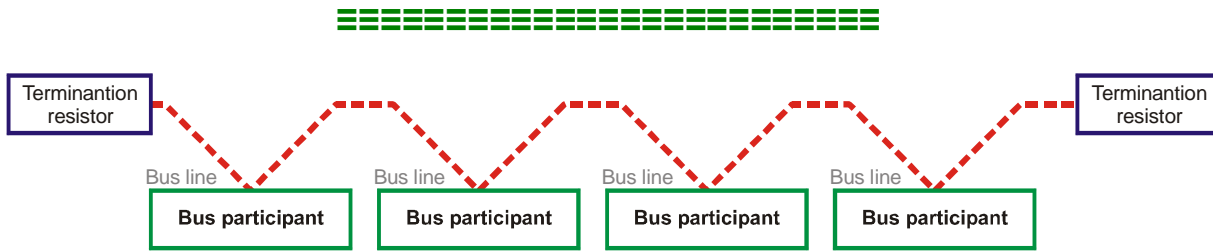
Figure 1-3: CAN bus topology
