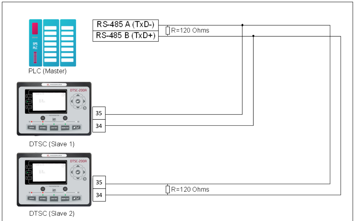
Figure 1-2: Interface overview - serial interface Modbus half-duplex
