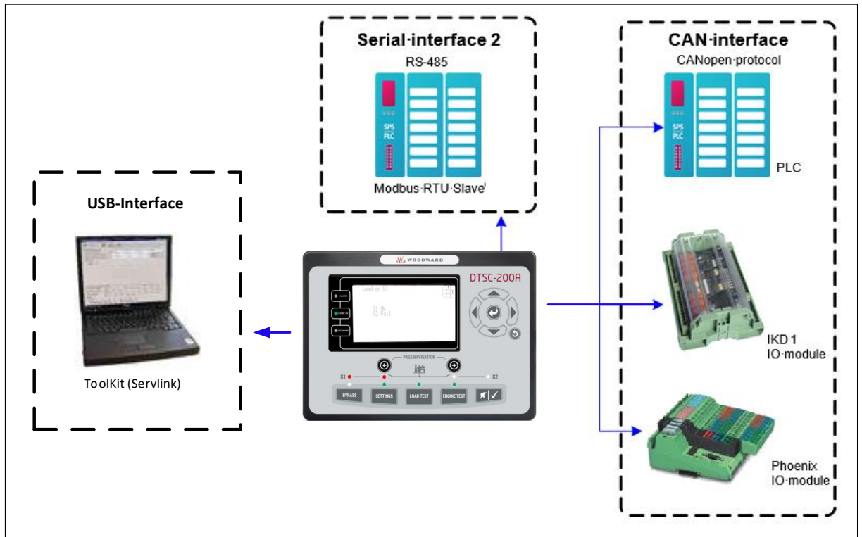
Figure 1-1: Interface overview
