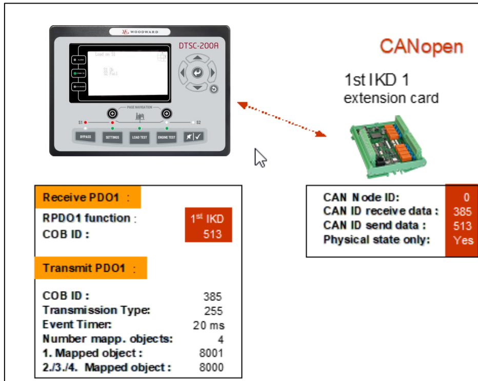
Figure 4-4: CANopen Interface – Adjustments for external devices
