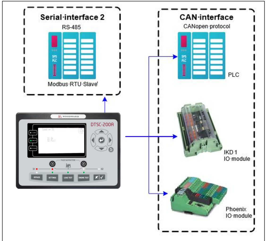
Figure3-1: Serial interface - overview
