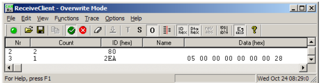
Figure 4-17: Cyclical sending of data - reply
