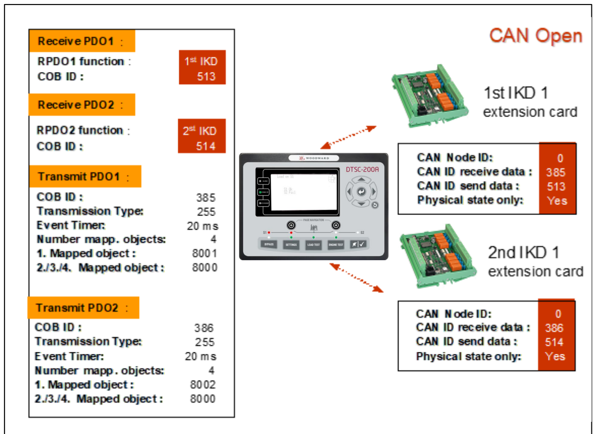
Figure 4-5: CANopen interface - expansion with two IKD 1
