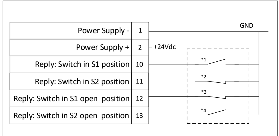
Figure 3-2: Limit switch reply wiring - all replies
