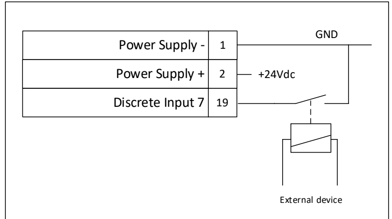
Figure 5-3: Example - transition mode selection switch wiring
