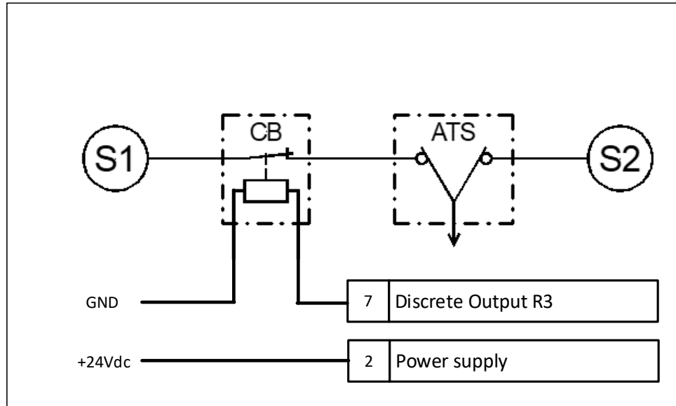
Figure 5-5: Example - Shunt trip enable signal wiring
